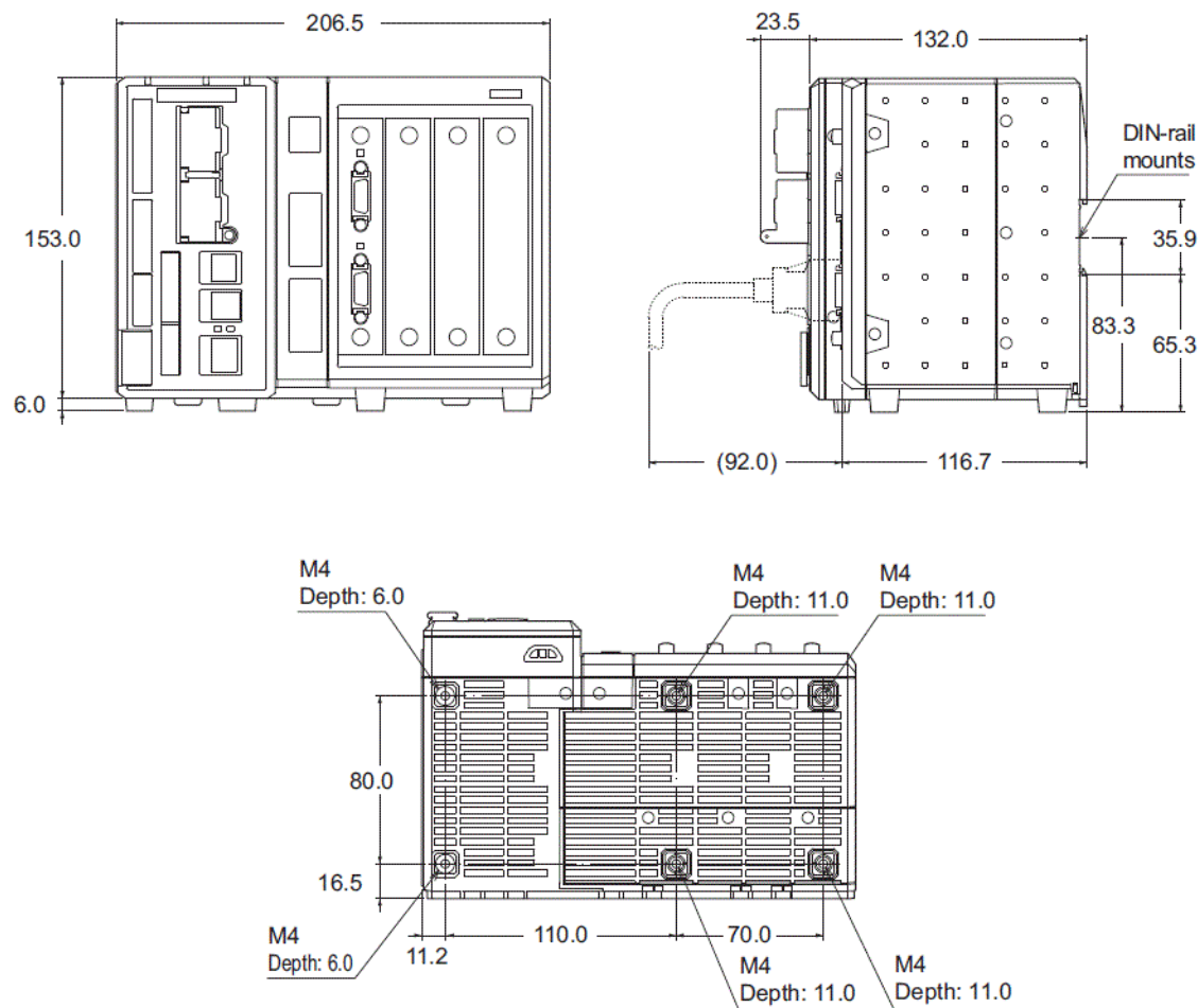
Controller Unit (XG-8800L) With one camera input unit XG-EC80 installed (factory default state)
