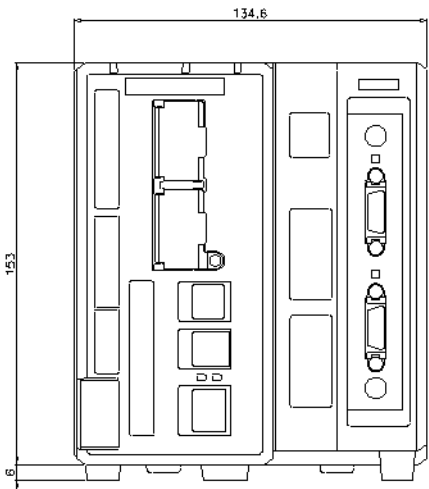
Controller unit
