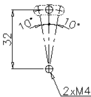
Screw hole dimensions
