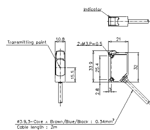
Transmitter
