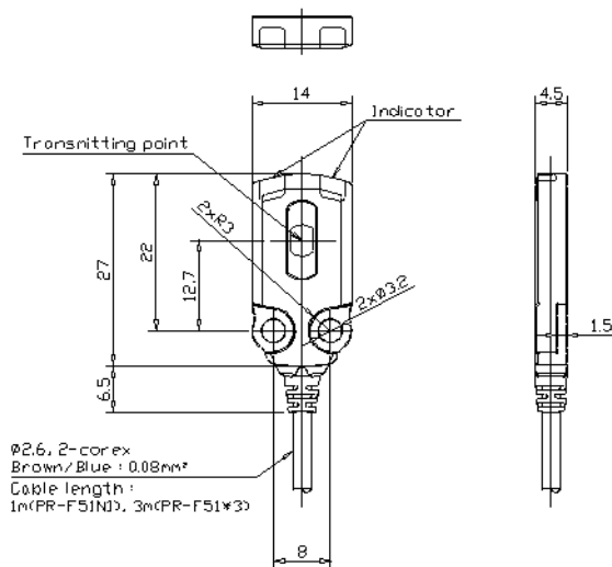
Transmitter
