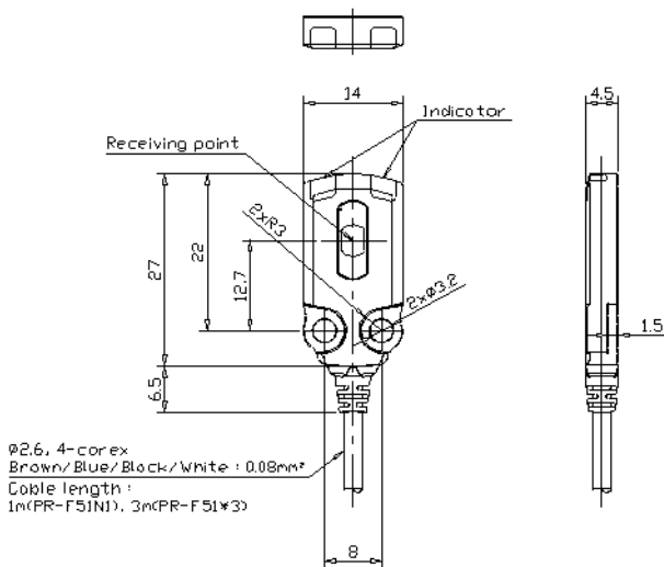
Receiver
