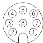
Pin arrangement
