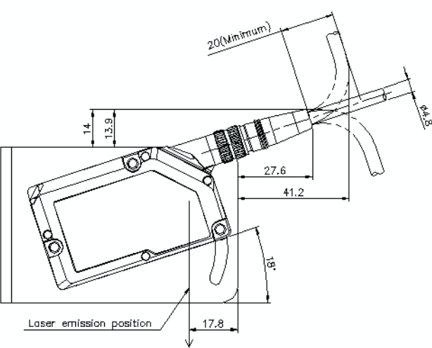
With vertical diagonal mounting bracket(OP-88345):Line mode,Laser vertical mounting 150mm
