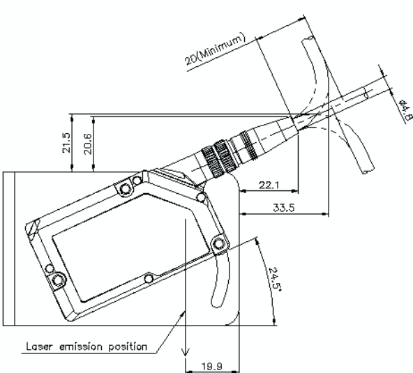
With vertical diagonal mounting bracket(OP-88345): Line mode,Laser vertical mounting 80mm
