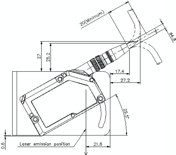
With vertical diagonal mounting bracket(OP-88345): Line mode,Laser vertical mounting 55mm
