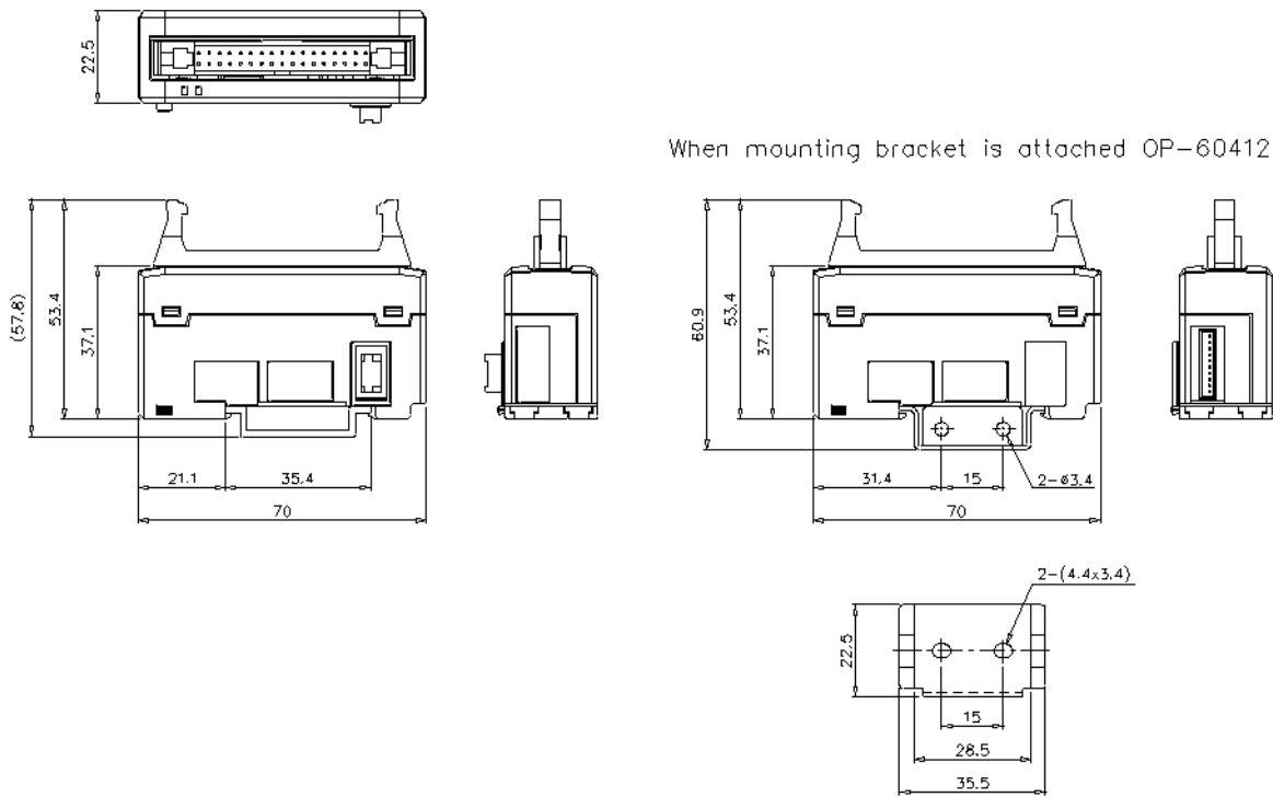
DIN-rail mounting
