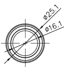
O-ring for left
