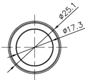
O-ring for right
