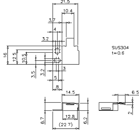
Mounting bracket
