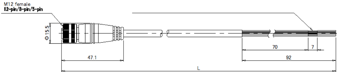
M12 5-pin female
