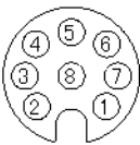
Pin arrangement
