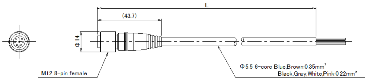
Pin arrangement
