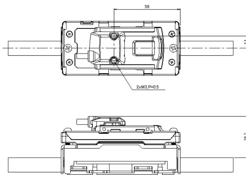
detection head
