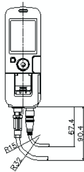
When power supply and Ethernet cable are connected
