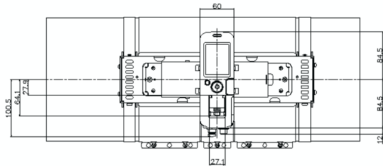
When FD-G is installed as horizontal integrated system
