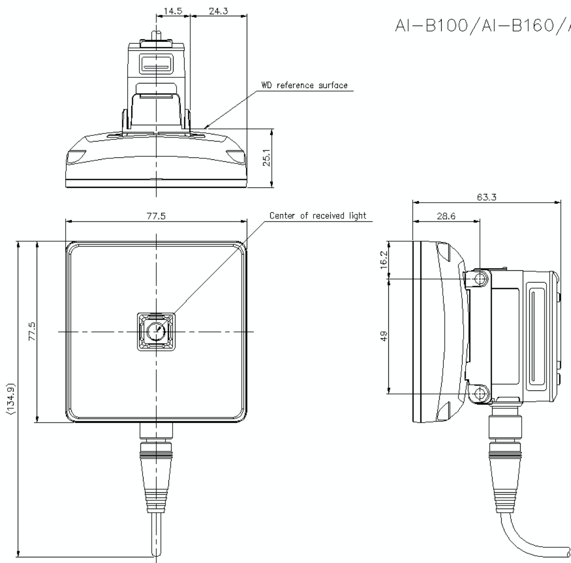
aib100_160_d32b_dimension_01.gif
