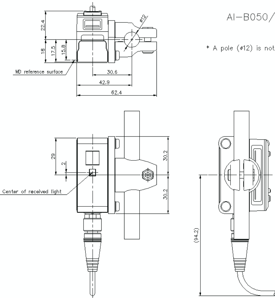
aib050_100_88116_dimension_01.gif
