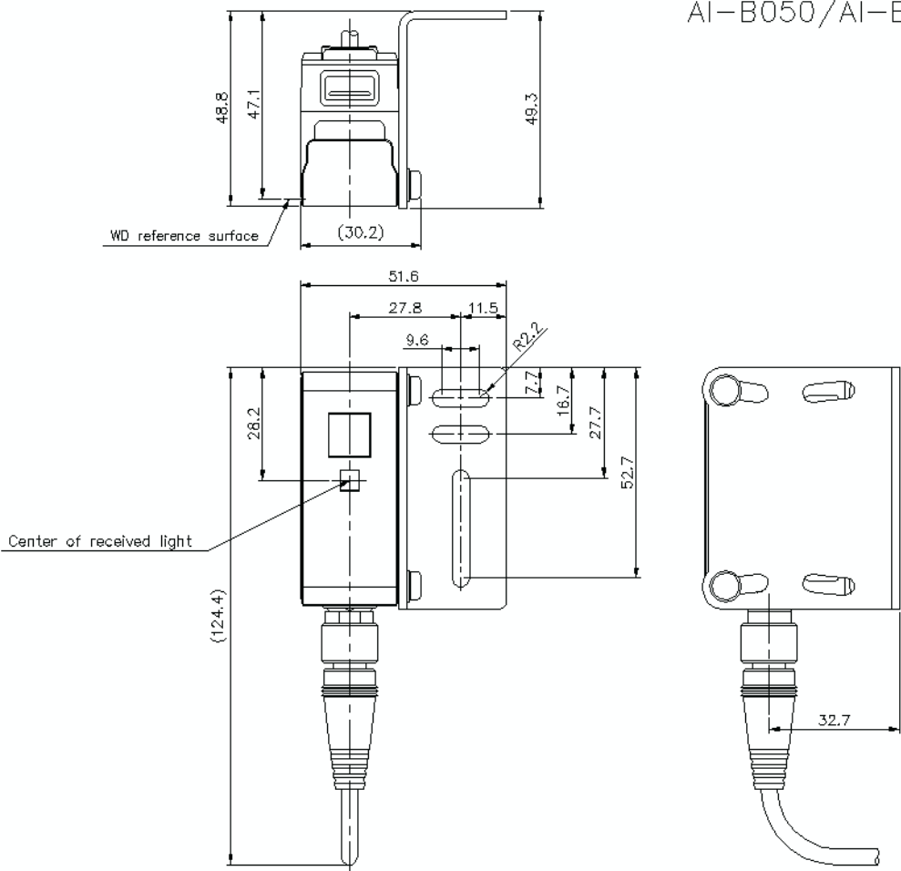
aib050_100_88115_dimension_01.gif
