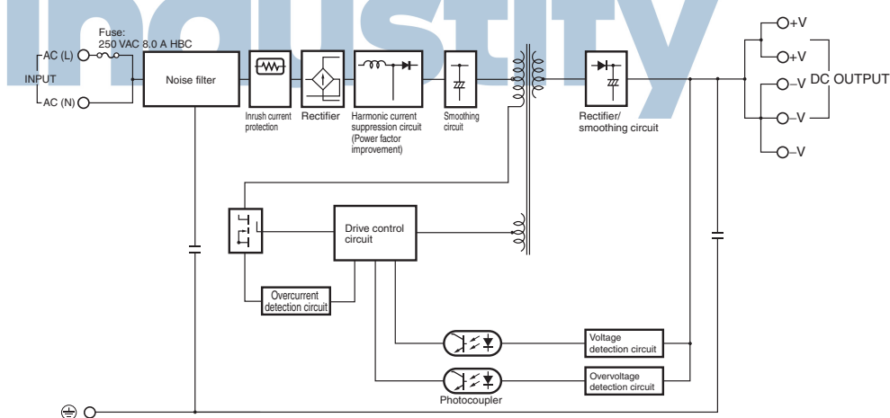
S8VK-C24024 (240W)
