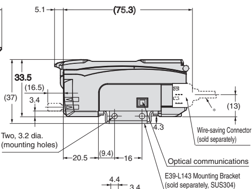
Mounting Holes
